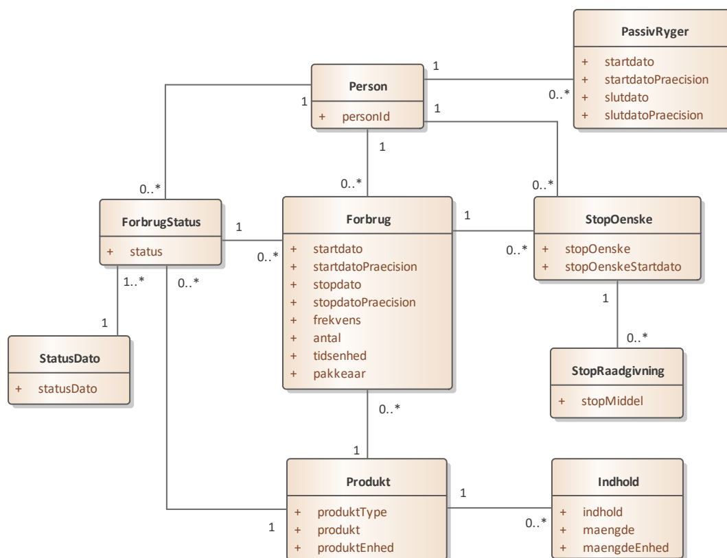
Figur 2 Informationsmodel
